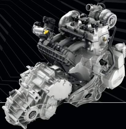
Rotax ACE triple-cylinder engine
